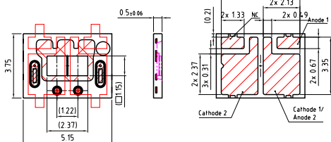
Component Location on Pad
