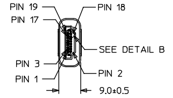
HDMI(M)
