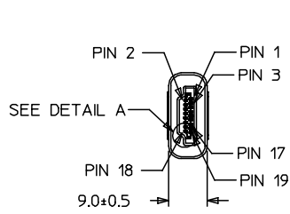
HDMI(M)
