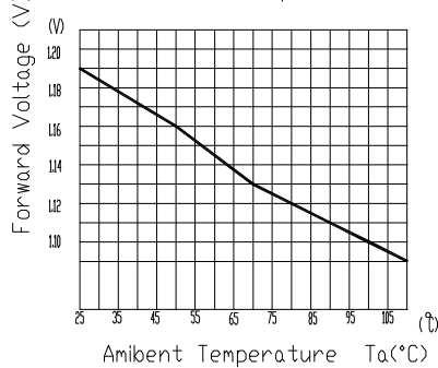
Fig. 5 Forward Voltage vs. Ambient Temperature
