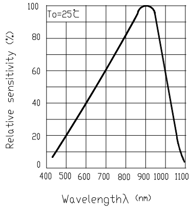
Fig.3 Spectral Sensitivity
