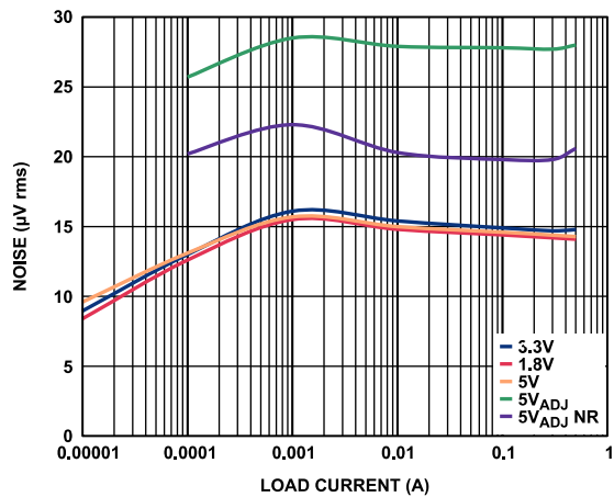
Figure 48. Output Noise vs. Load Current and Output Voltage, C_{OUT} = 1\ \mu\text{F}
