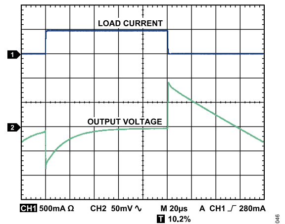
Figure 51. Load Transient Response, C_{IN} = C_{OUT} = 1\ \mu\text{F} , I_{LOAD} = 1\text{ mA to } 500\text{ mA} , V_{OUT} = 3.3\text{ V} , V_{IN} = 5\text{ V}
