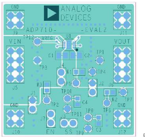
Figure 78. Example LFCSP PCB Layout
