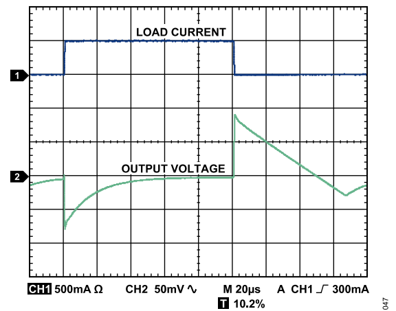
Figure 52. Load Transient Response, C_{IN} = C_{OUT} = 1\ \mu\text{F} , I_{LOAD} = 1\text{ mA to } 500\text{ mA} , V_{OUT} = 5\text{ V} , V_{IN} = 7\text{ V}
