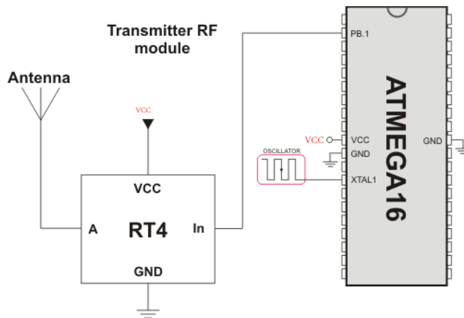
Simple Transmitter connection
