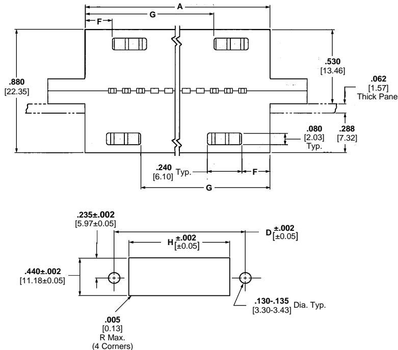
Recommended Panel Cutout
