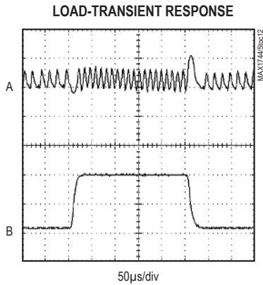
V_{IN} = 7.2\text{V} , V_{OUT} = 3.3\text{V} , LOAD CURRENT = 0.1A TO 2A A: V_{OUT} , 50mV/div, 3.3V AC-COUPLED B: LOAD CURRENT, 1A/div
