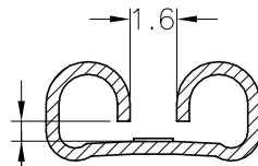
SECTION C-C
