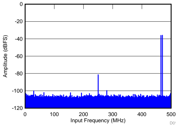
f_{\text{IN1}} = 470 \text{ MHz} , f_{\text{IN2}} = 465 \text{ MHz} , each tone at -36 dBFS, IMD = 109.2 dBFS
