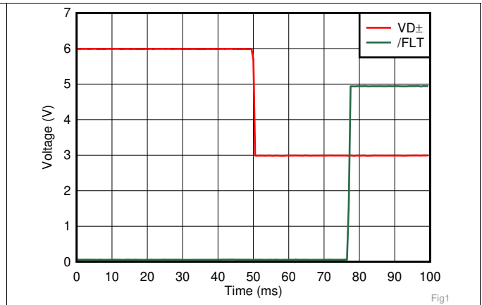
Figure 15. FLT Recover Time After OVP Clear
