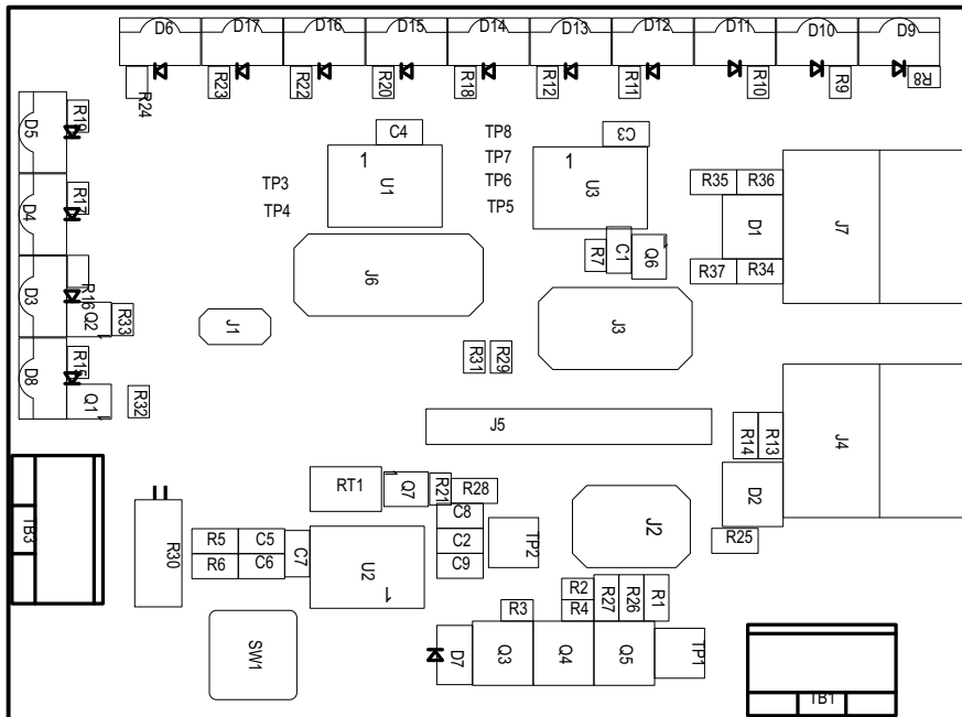
Figure 4-2. Top Assembly
