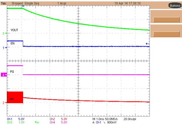
Figure 15. Power Down Sequence and Active Output Discharge ( V_{IN} = 3.6\text{ V} , V_{OUT} = 1.8\text{ V} , I_{OUT} = 0\text{ A} , L = 1\ \mu\text{H} , C_{OUT} = 10\ \mu\text{F} )
