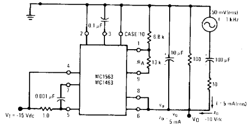
FIGURE 8 - SHUTDOWN CURRENT
