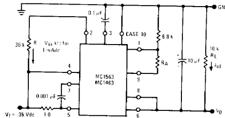
FIGURE 8 - SHUTDOWN CURRENT
