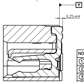
SECTION Z-Z (SCALE 10:1)
