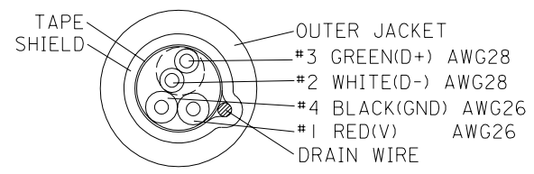
CABLE CONSTRUCTION
