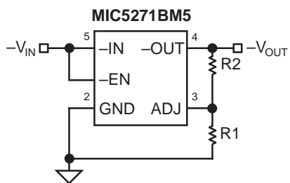
Figure 1. Adjustable Voltage Application
