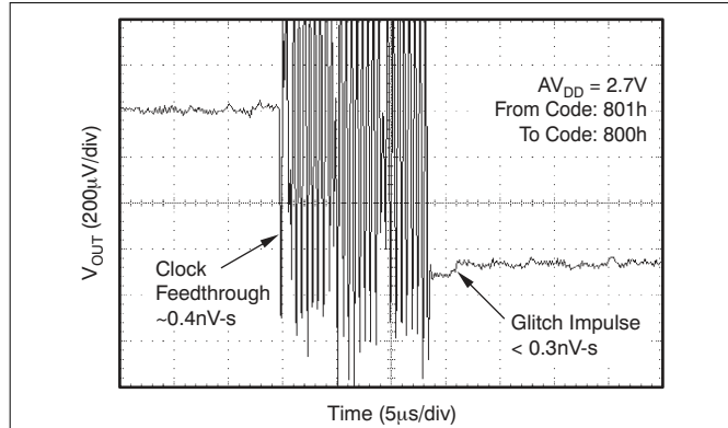
Figure 7-68. Glitch Energy, 2.7-V, 12-Bit, 1-LSB Step, Falling Edge
