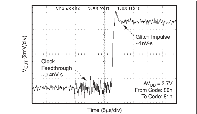
Figure 7-69. Glitch Energy, 2.7-V, 8-Bit, 1-LSB Step, Rising Edge
