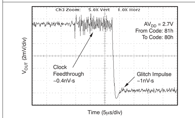
Figure 7-68. Glitch Energy, 2.7-V, 12-Bit, 1-LSB Step, Falling Edge
