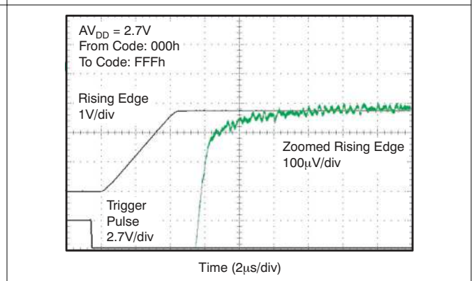
Figure 7-71. Full-Scale Settling Time, 2.7-V Rising Edge
