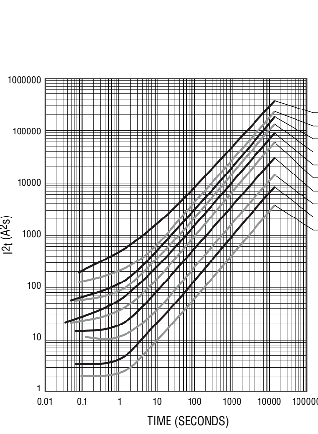
Average I²t vs. t Curves
