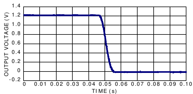
FIGURE 11. RAMP DOWN
