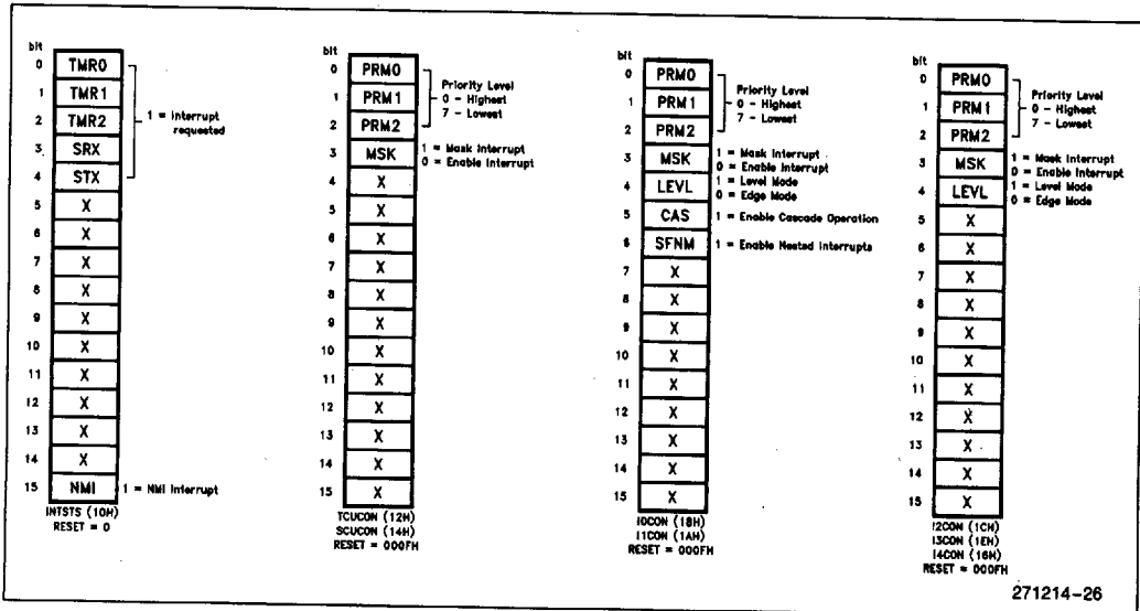
Figure 28. Interrupt Control Unit Registers
