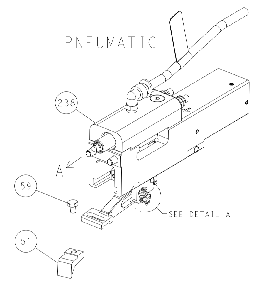
FEED SPRING SETTING POSITION DETAIL A
