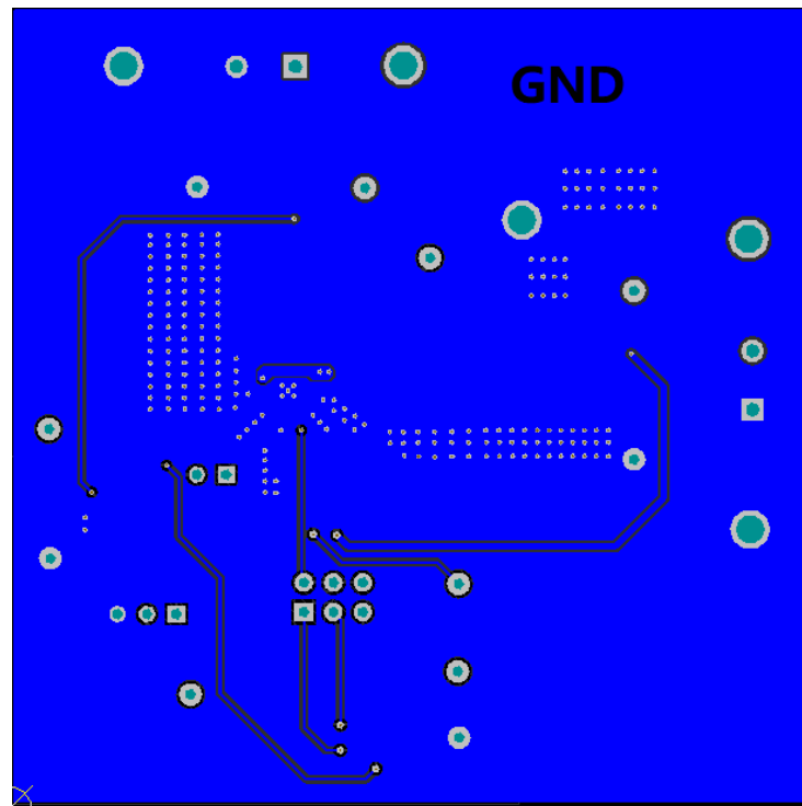
Figure 4-5. Bottom Layer
