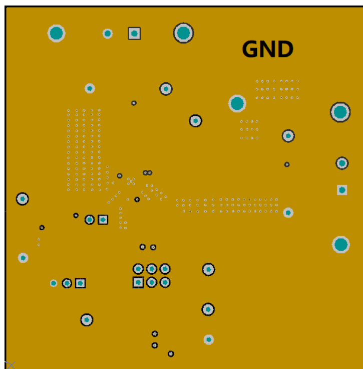
Figure 4-3. Internal Layer1
