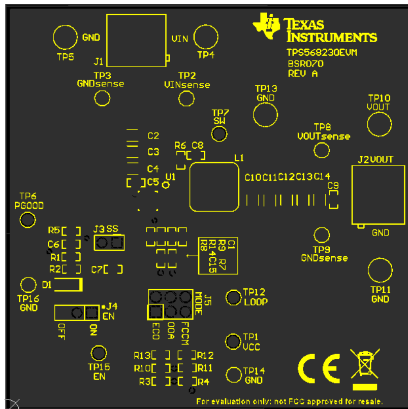
Figure 4-1. Component Placements
