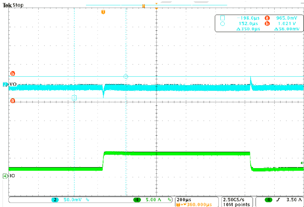
Figure 6-10. Load Transient from 2 A to 6 A
