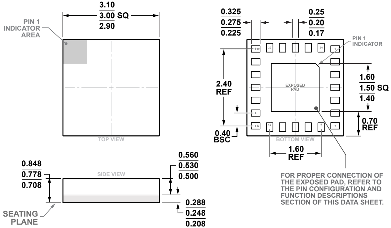
Figure 28. 24-Terminal Land Grid Array [LGA] 3 mm x 3 mm Body and 0.780 mm Package Height (CC-24-14) Dimensions shown in millimeters
