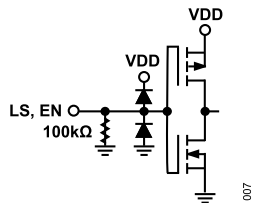
Figure 7. LS and EN Control Interface Schematic
