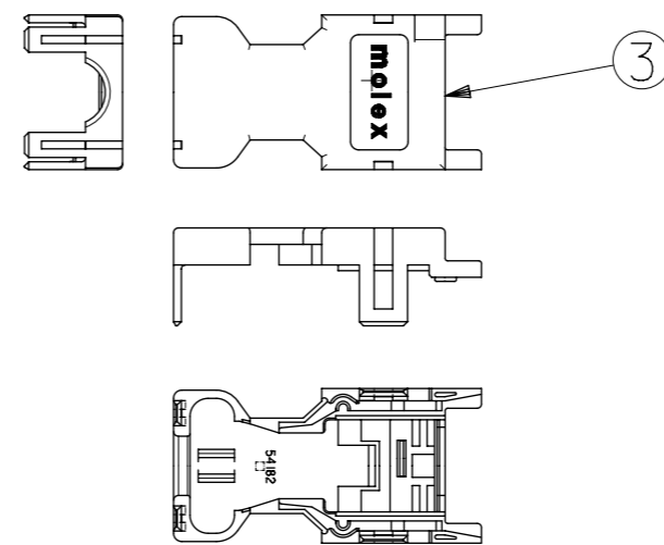
COVER B
