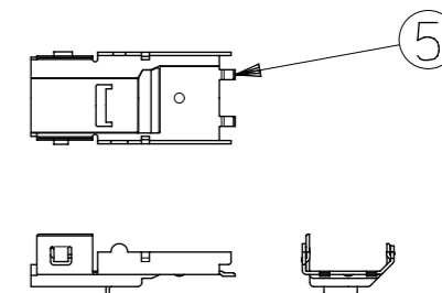
SHELL BODY
