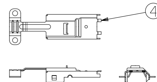
SHELL COVER
