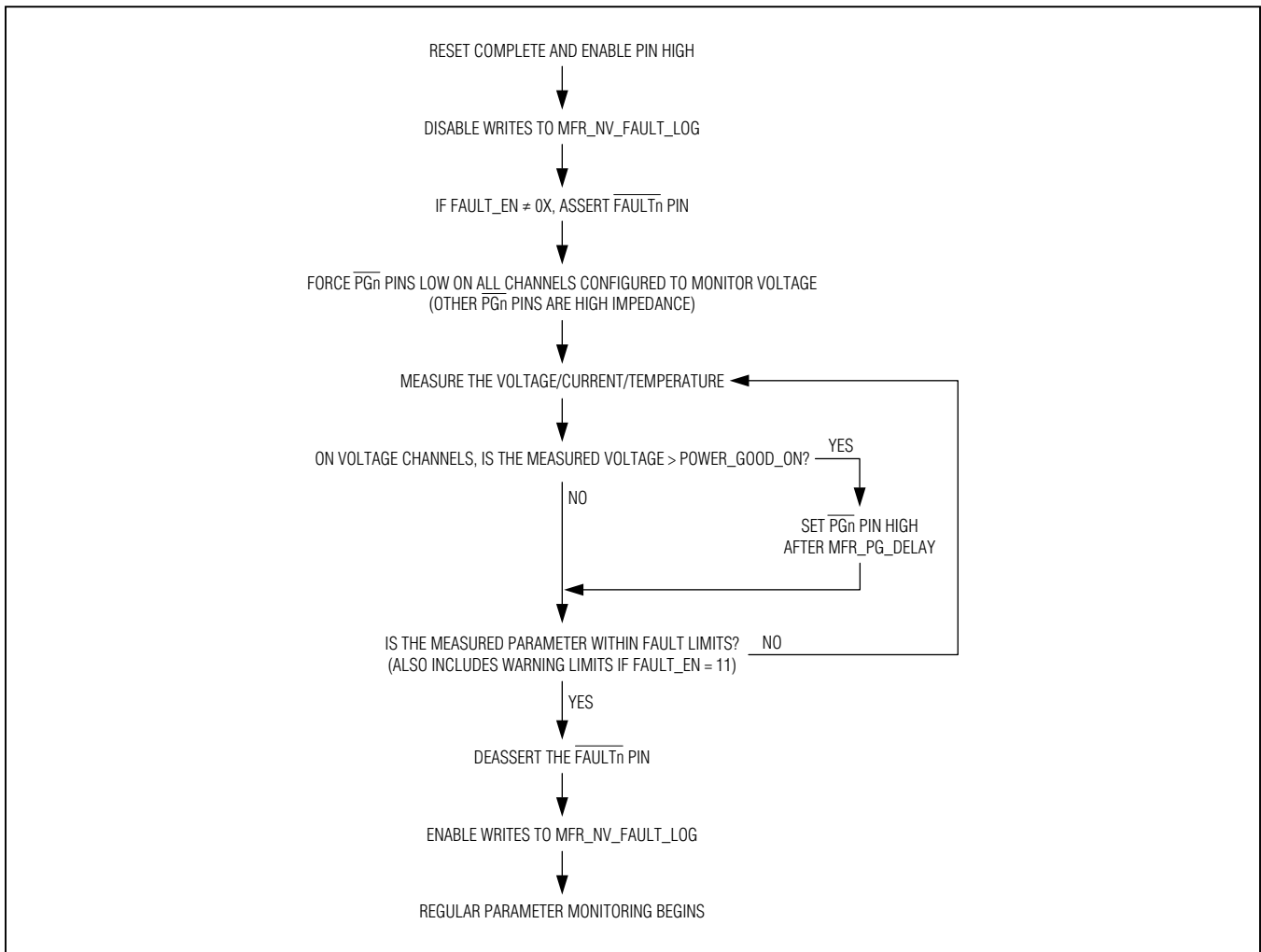
Figure 1. \overline{PGn} and \overline{FAULTn} Output After a Channel is Enabled
