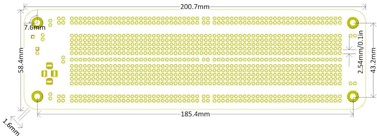
Figure 6: Dimensions of the Proto-Full PCB.
