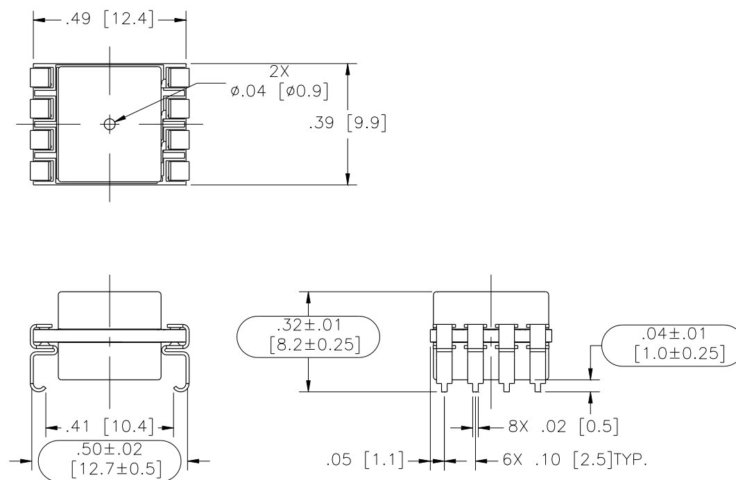
Model: MS4525-MMvoxxxS
