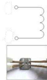
Figure 1. DCR test
