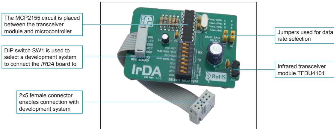
Figure 1: IrDA board
