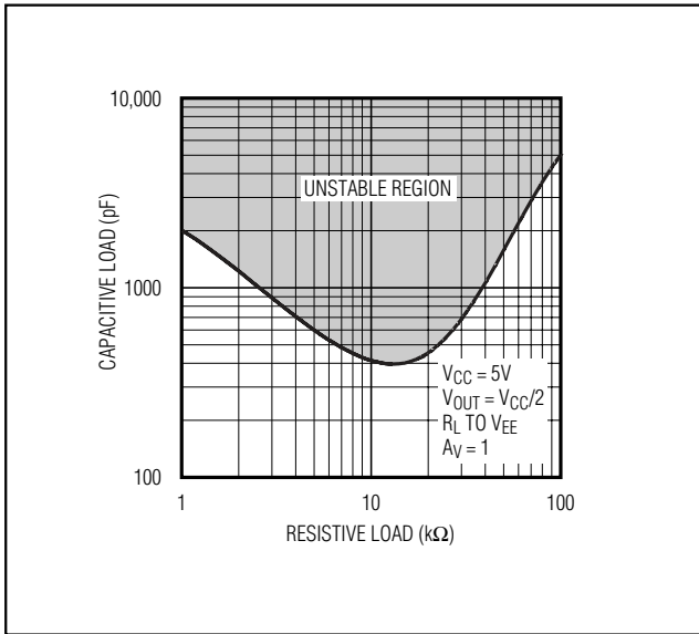
Figure 4. Capacitive-Load Stable Region Sourcing Current
