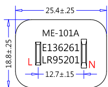
ME-101A (NEMA 1-15P) (Dimensions of Plug Face)
