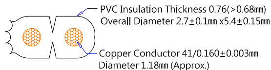
SPT-1 18AWGx2C截面圖 (Wire Cross-Section)
