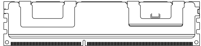
Figure 1: 240-Pin RDIMM (MO-269 R/C H)
