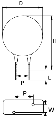
Two-Terminal Type
