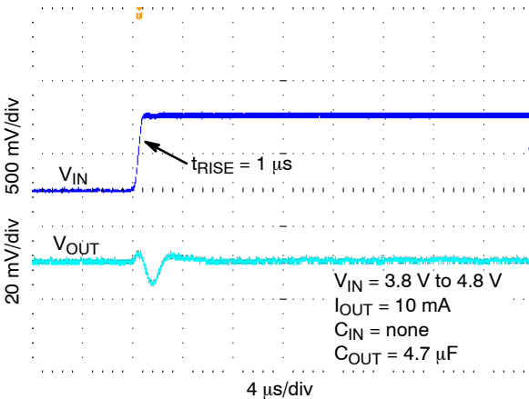
Figure 34. Line Transient Response – Rising Edge, V_{OUT} = 3.3\text{ V} , I_{OUT} = 10\text{ mA} , C_{OUT} = 4.7\text{ }\mu\text{F}
