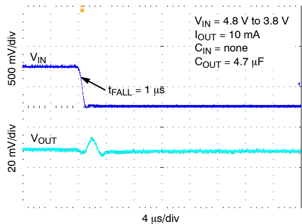
Figure 35. Line Transient Response – Falling Edge, V_{OUT} = 3.3\text{ V} , I_{OUT} = 10\text{ mA} , C_{OUT} = 4.7\text{ }\mu\text{F}
