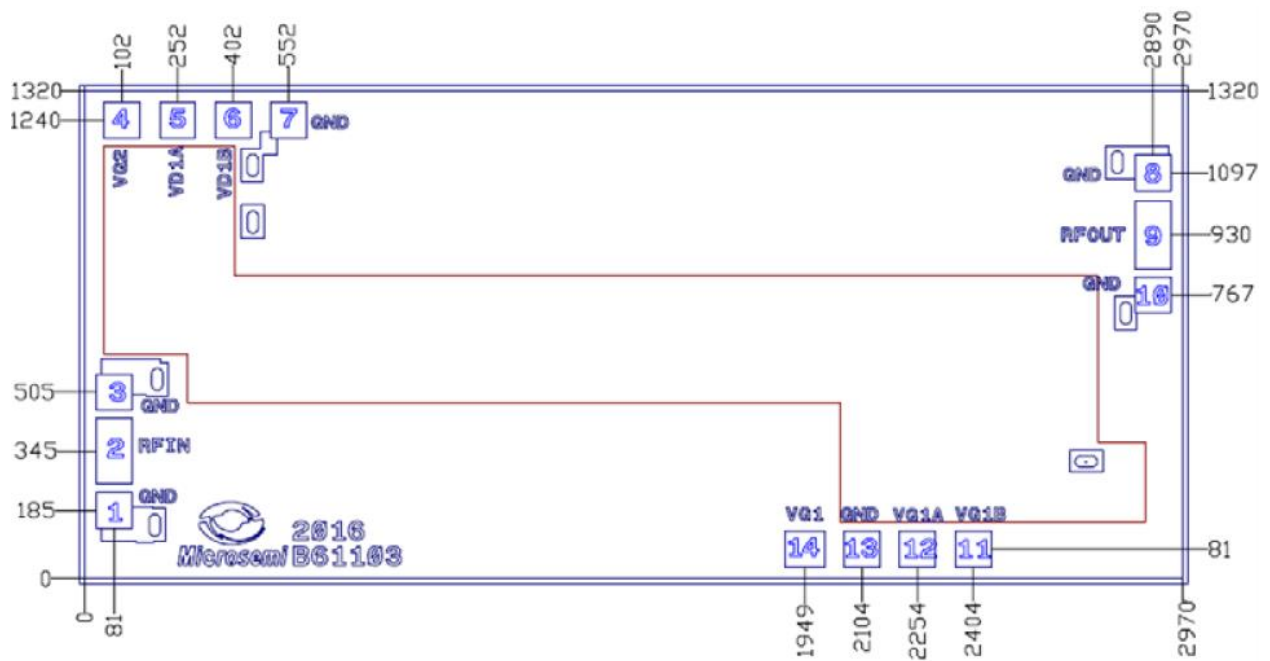
Figure 15 Chip Outline
