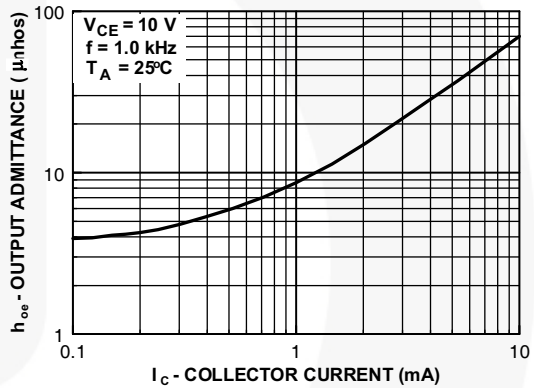
Figure 16. Output Admittance
