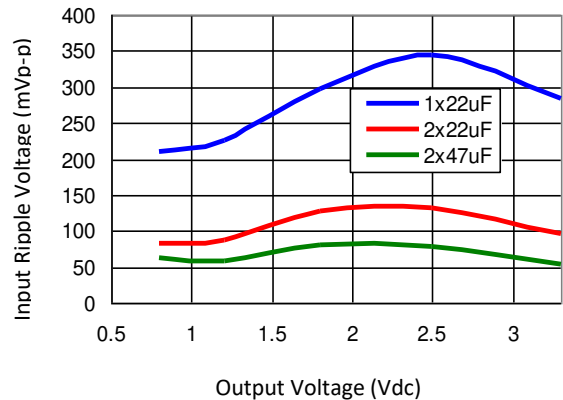
Figure 28. Input ripple voltage for various output voltages with 1 \times 22\mu F , 2 \times 22\mu F or 2 \times 47\mu F ceramic capacitors at the input (30A load). Input voltage is 12V.
