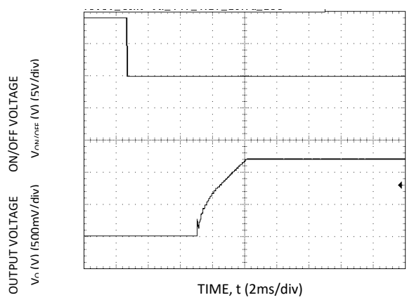
Figure 9. Typical Start-up Using On/Off Voltage ( I_o = I_{o,max} ).
