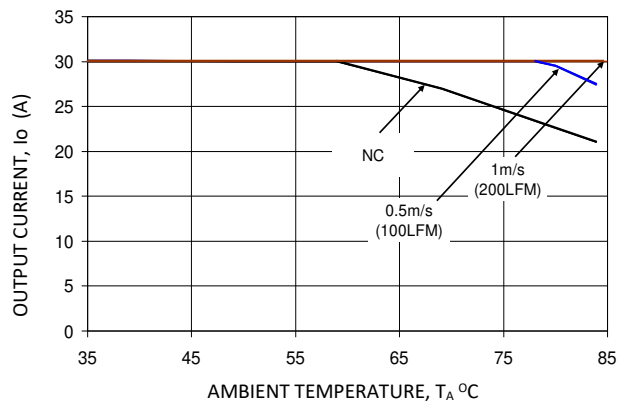
Figure 10. Output Current Derating versus Ambient Temperature and Airflow at 12V in.
