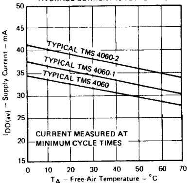
AVERAGE CURRENT vs TEMPERATURE
