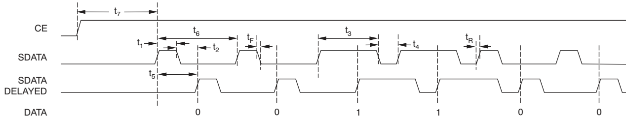
Figure 2. SDATA/CE Timing
