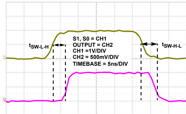
FIGURE 29. CHANNEL TO CHANNEL SWITCHING TIME
