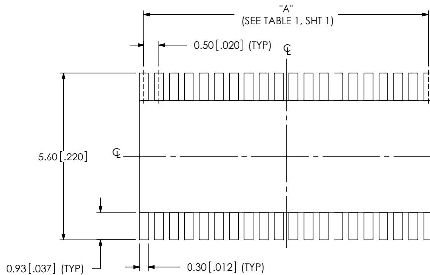
FIG 2 -20 POS SHOWN
