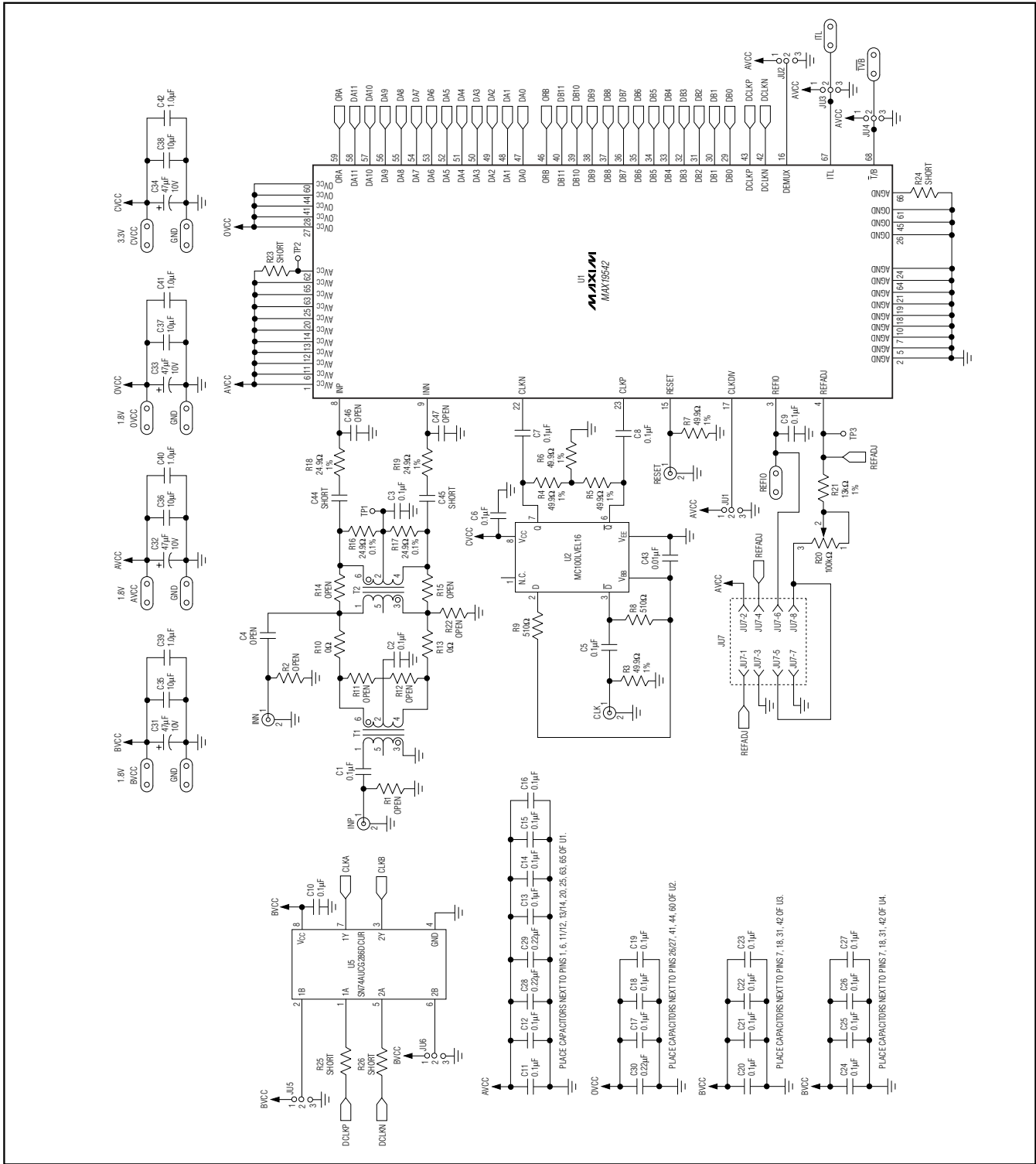
Figure 1b. MAX19541/MAX19542 EV Kits Schematic (Sheet 2 of 3)
