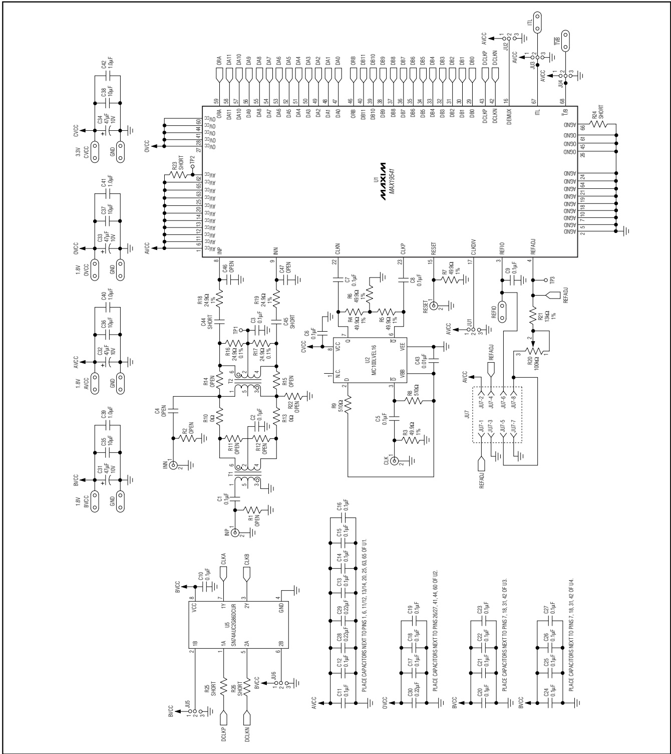
Figure 1a. MAX19541/MAX19542 EV Kits Schematic (Sheet 1 of 3)
