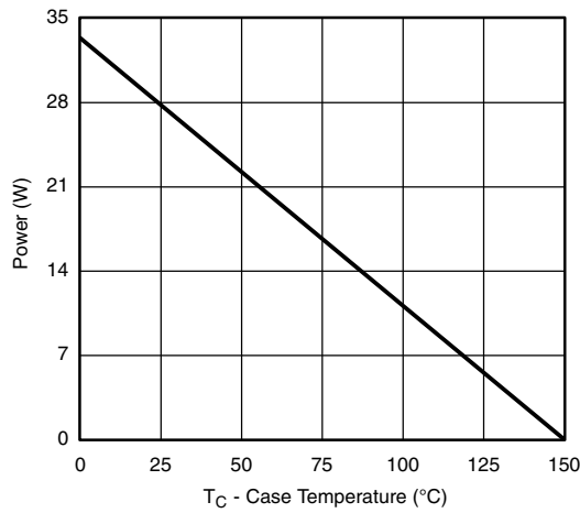
Power, Junction-to-Case
