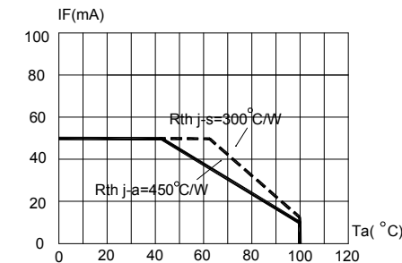
FIG.4a RED MAXIMUM FORWARD DCCURRENT VS AMBIENT TEMPERATURE ( T_{jmax}=110^{\circ}C )
