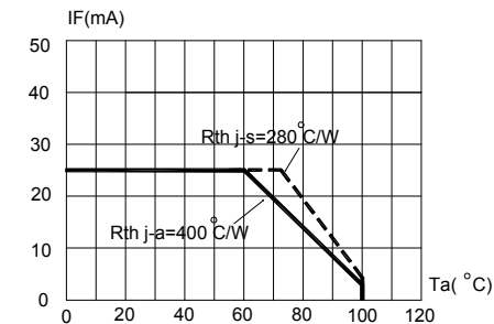
FIG.4b GREEN MAXIMUM FORWARD DCCURRENT VS AMBIENT TEMPERATURE ( T_{jmax}=110^{\circ}C )
