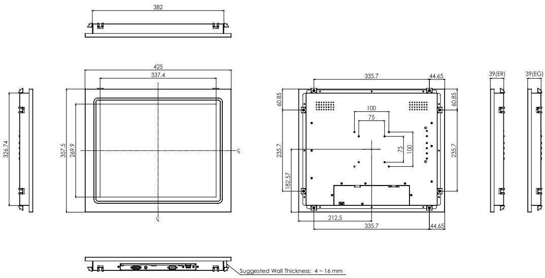
Figure 2.2 IDS-3217E Series Dimensions
