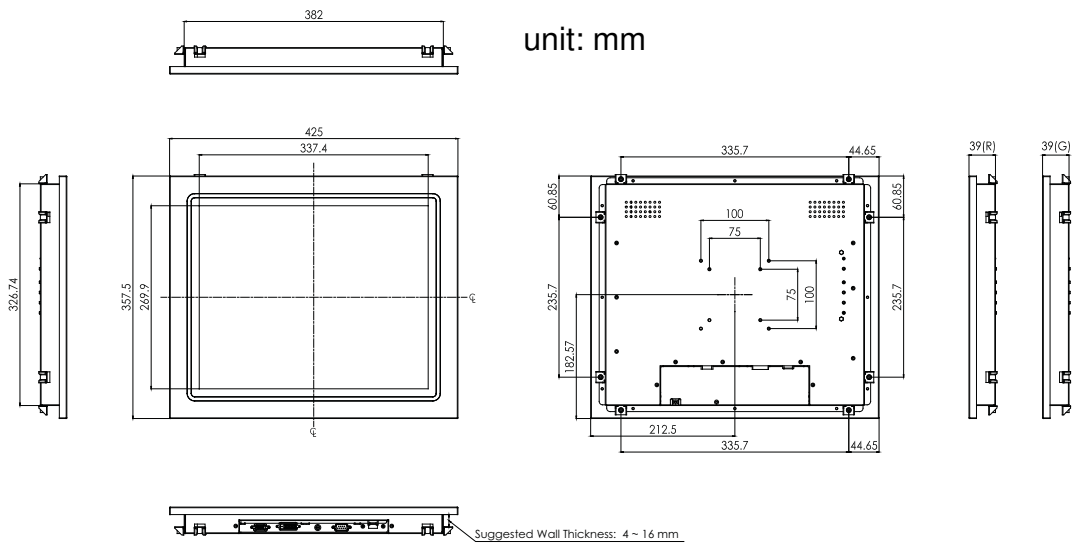
Figure 2.1 IDS-3217 Series Dimensions
