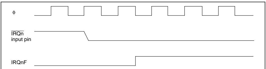
Figure 5.4 Timing of \text{IRQnF} Setting
