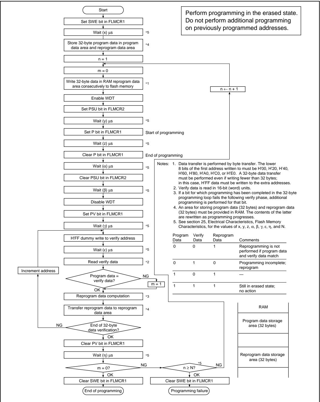
Figure 21.12 Program/Program-Verify Flowchart
