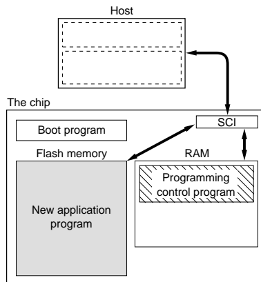
Figure 21.4 Boot Mode
