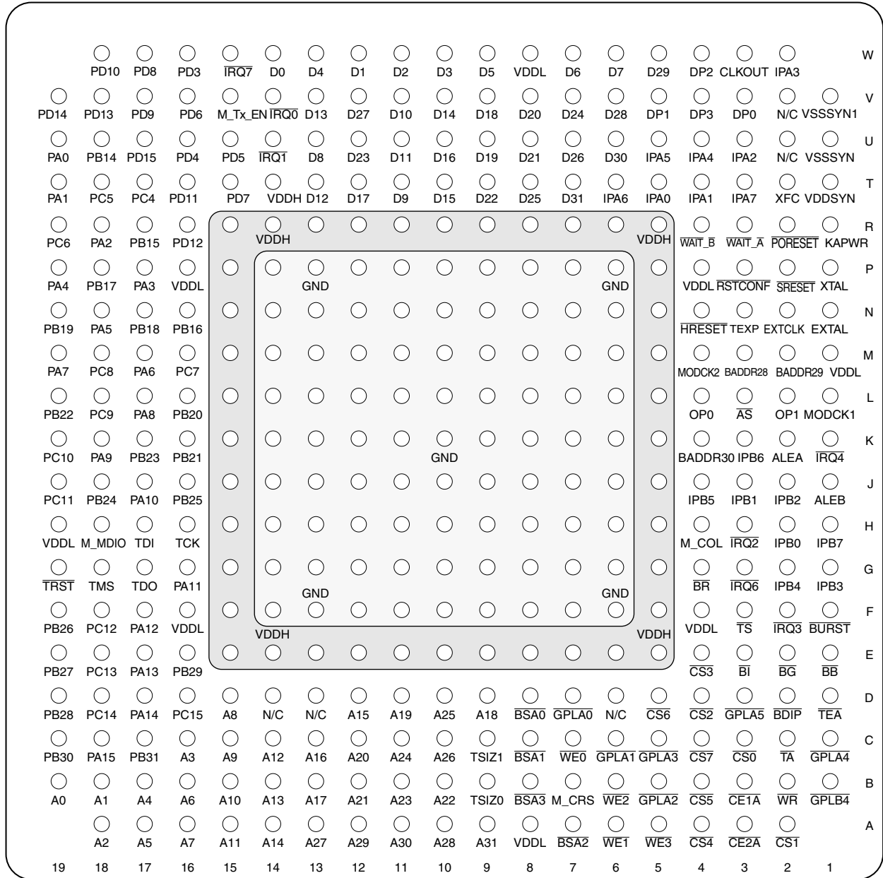
Figure 74. Pinout of the PBGA Package
