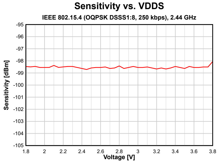
Figure 8-16. Sensitivity vs. Supply Voltage (VDD5) (250 kbps, 2.44 GHz)
