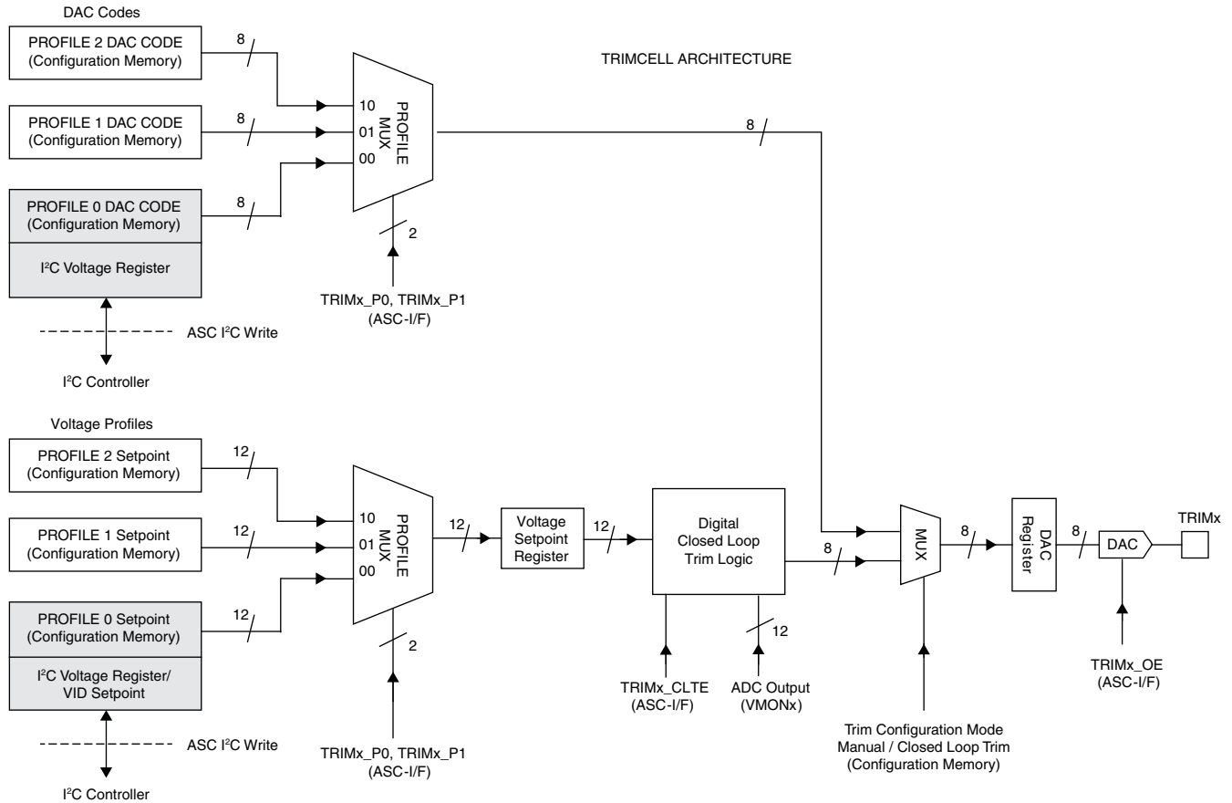
Figure 26. TrimCell Architecture
