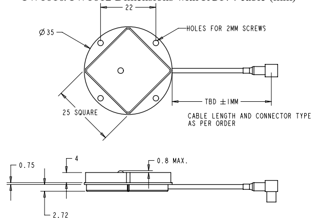
TW1010/TW1012 Dimensions with RG174 cable (mm)
